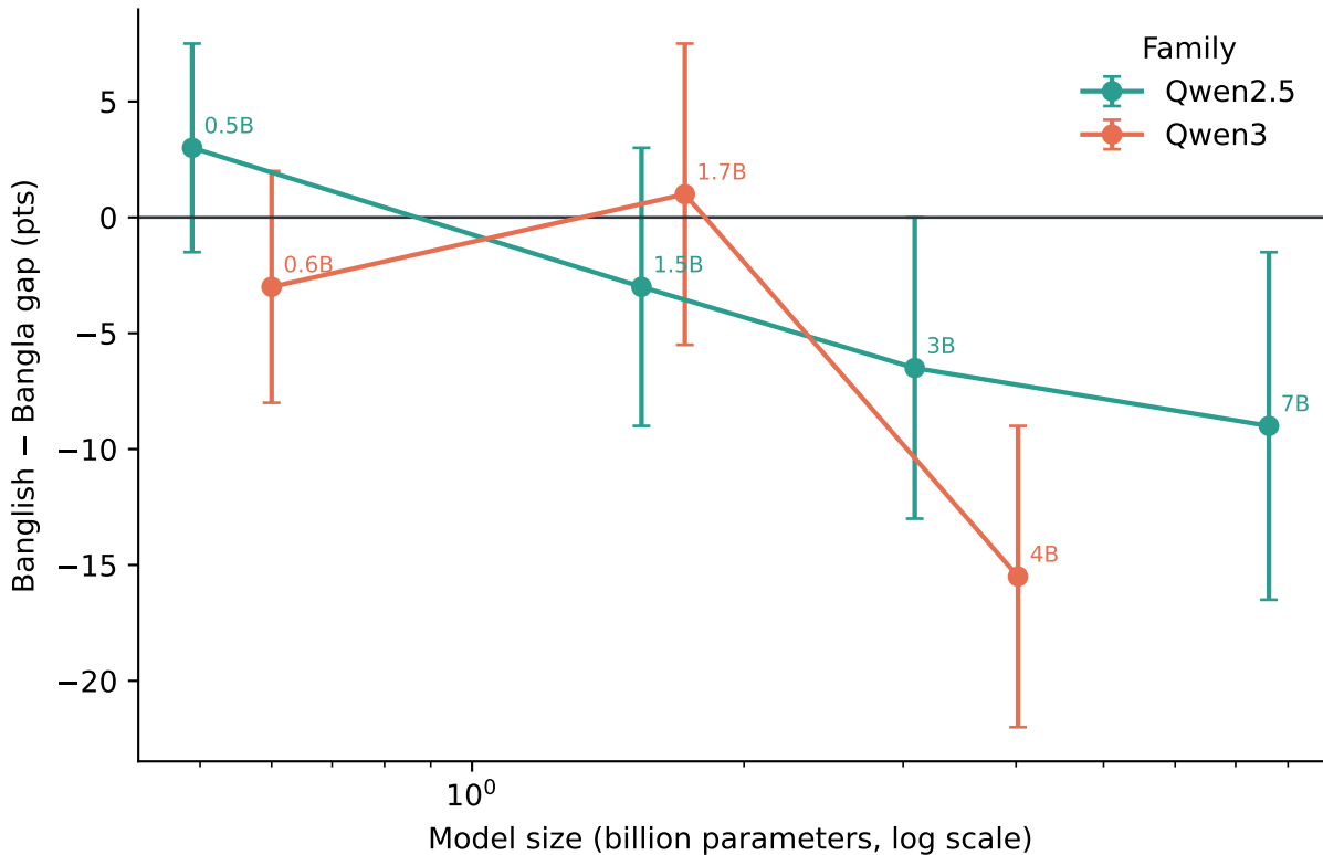
Within-family scaling: the Banglaj gap widens with model size
